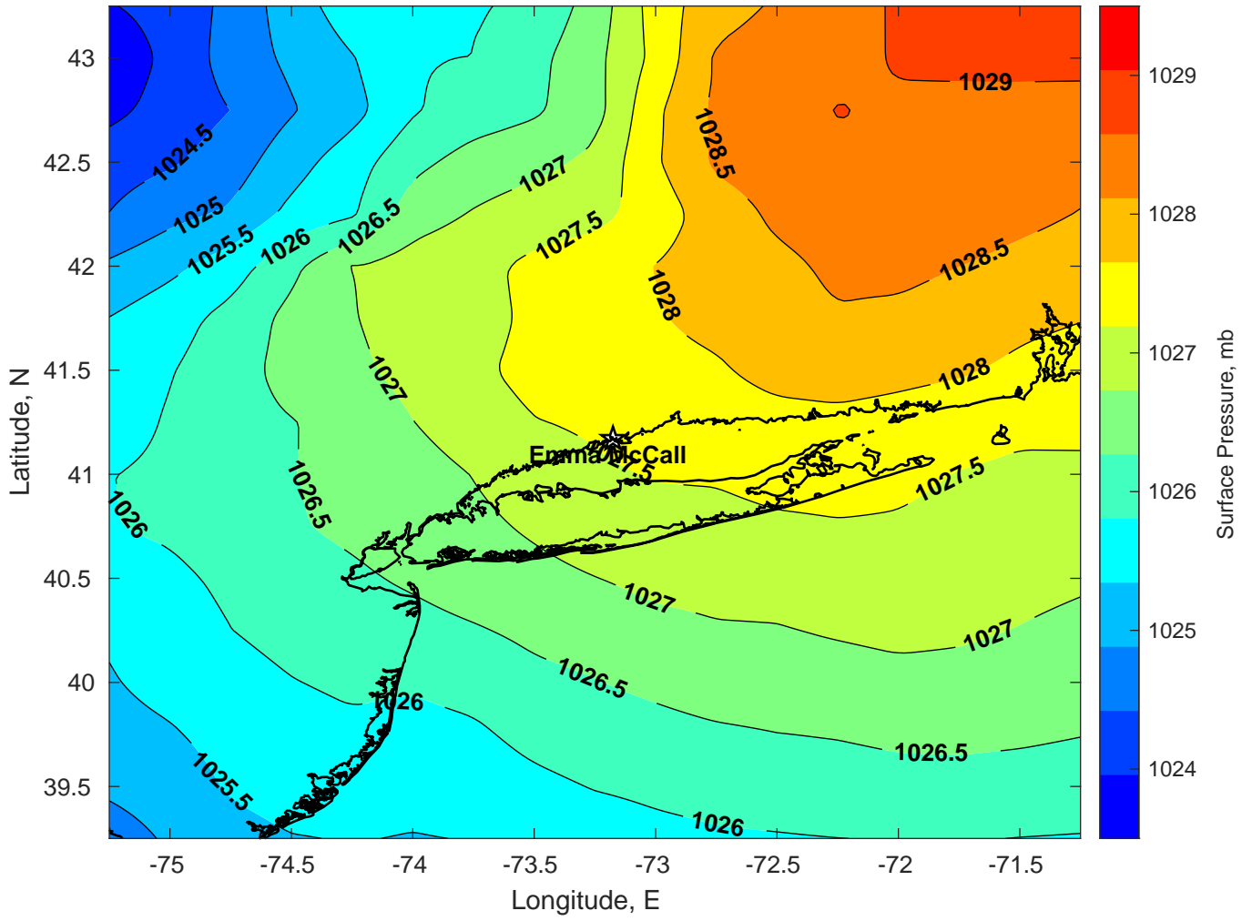
Surface Pressure (mb) for Emma McCall at 05-May-2024 06:00:00
